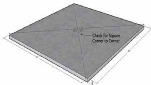
SLAB MUST BE LEVEL & SQUARE
